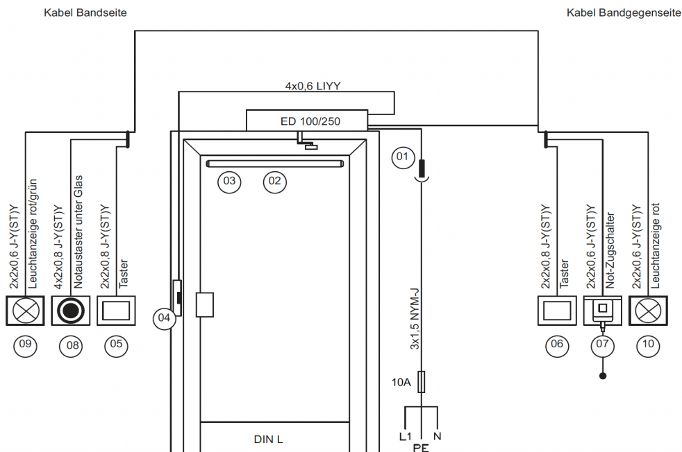
Skizze Behinderten WC (laut System 3)
