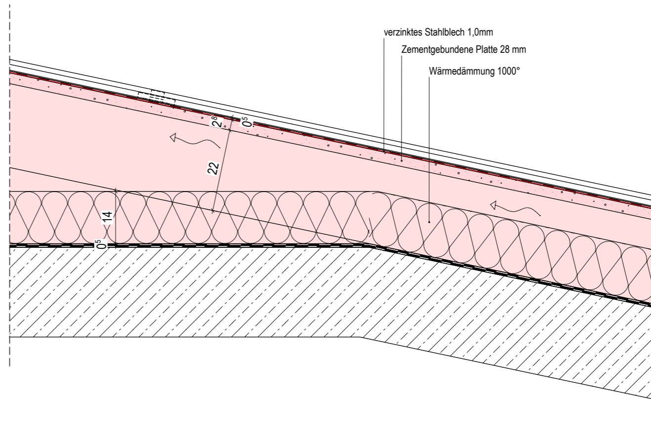
SCHITT parallel zur BRANDWAND
