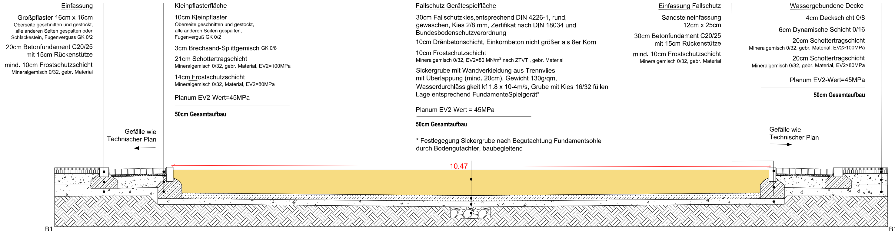
Detail B1: Schaukel M 1:40
